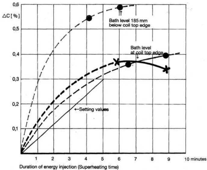
Fig. 14: Carburization velocities in a 6 t induction furnace of 2600 kW and 230 Hz
