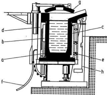
Figure 112. Layout of an induction crucible furnace [82]
