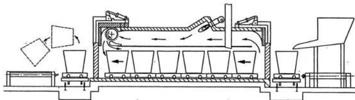
Figure 110. Pre-heating and drying of the charge for induction crucible furnaces; System: gas-fired push-through furnace system (500 °C) with high gas circulation, especially for the pre-heating of magnetic yokes. Furnace time about 60 min., core temperature of the magnetic yokes 200 °C, charge weight of the furnace 2 t, throughput 2 \times 2 \text{ t}/20 \text{ min.} = 12 \text{ t/h} .
