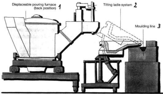
Fig. 13: Tilting ladle system with the PRESSPOUR® pouring furnace 1 travelling pouring furnace in retracted position 2 tilting ladle system 3 mould chain
