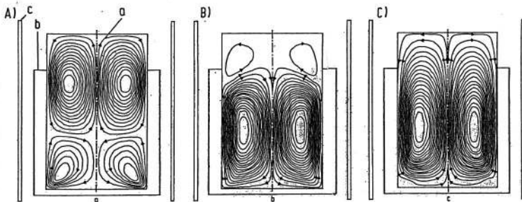
Figure 78. Flow field of a melt with single- and multiple-phase (travelling field) coil [73] A) single-phase coil, B) three-phase coil with travelling field direction from bottom to top, C) three-phase coil with travelling field direction from top to bottom. a - melt, b - coil, c - yoke
