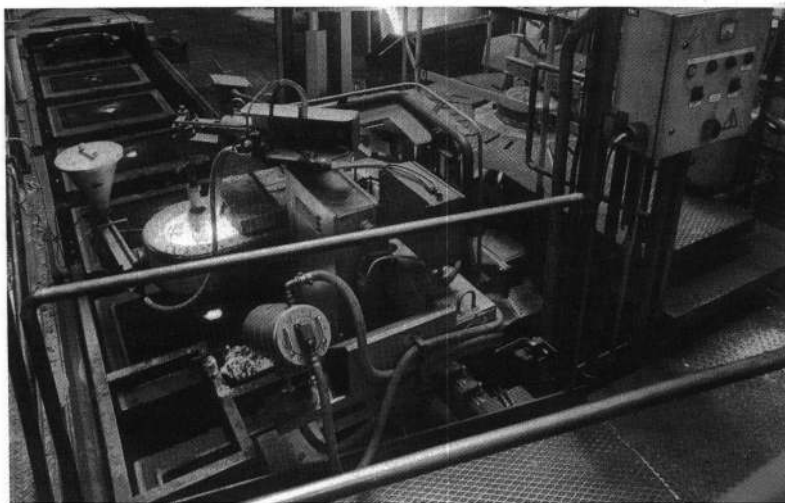
Fig. 17: 6-t PRESSPOUR ® pouring furnace with OPTIPOUR ® metal level control and inoculation system in operation at a Buderus moulding line.
