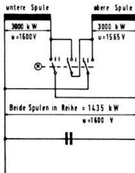
Figure 9: Circuit diagram of crucible-type storage furnace with reversible coil (Figure 8, right)
