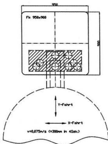
Fig. 2: Pouring field with the most frequently adopted casting positions.
