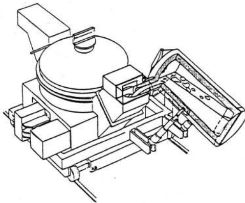
Figure 3: Converter (=transport ladle) in transfer position to casting furnace
