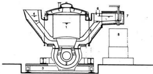
Figure 1: Schematic drawing of the pressurized gas-operated Pouromat OCC pouring system
