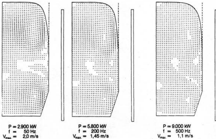
Fig. 13: Amount and direction of the melt flow in a 6 t coreless furnace
