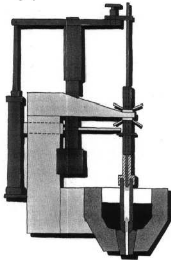
Fig. 10: ABB stopper mechanism with patented pouring nozzle cleaning device
