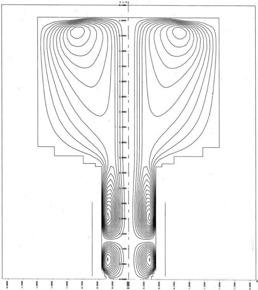
Fig. 3: Calculated metal flow
