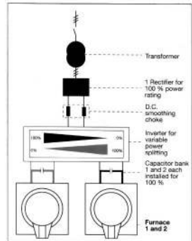
Figure 6: TWIN POWER circuit
