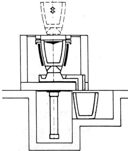
Figure 2: Cross-section through lifting crucible furnace for or 200 kg capacity.
