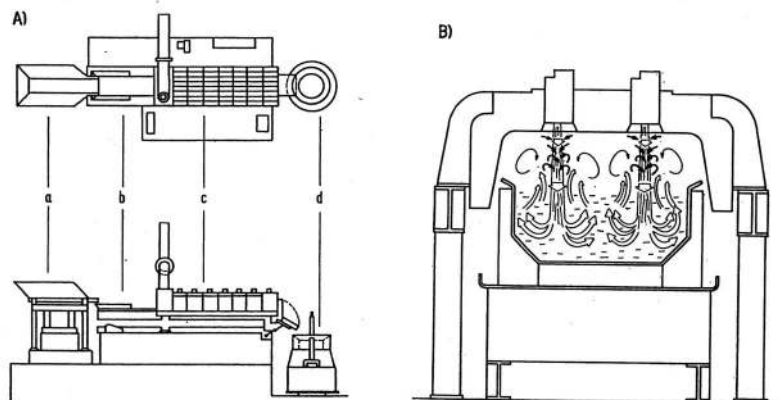
Figure 111. Pre-heating and drying of the charge for induction crucible furnaces; System: conveyor pre-heater [121]
