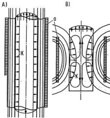
Figure 76. Principle of the induction crucible furnace [73] A) parallel magnetic field lines with infinitely extended coil and the resulting direction of forces. B) bent magnetic field lines with a finite coil and the resulting force components a - coil, K - force components
