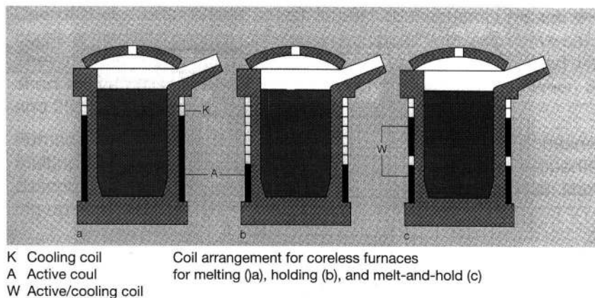
Fig. 8: Various types of a coreless holding furnace with different coil arrangements
