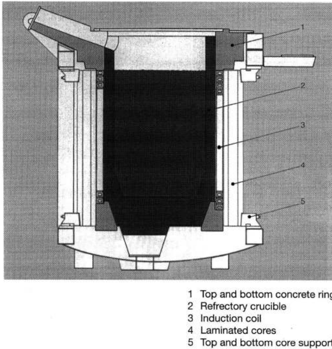
Fig. 9: Medium-frequency coreless furnace of type IFM as holding unit
