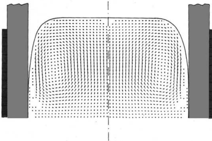
Fig. 15: Melt flow in a coreless induction furnace ITMK 6
