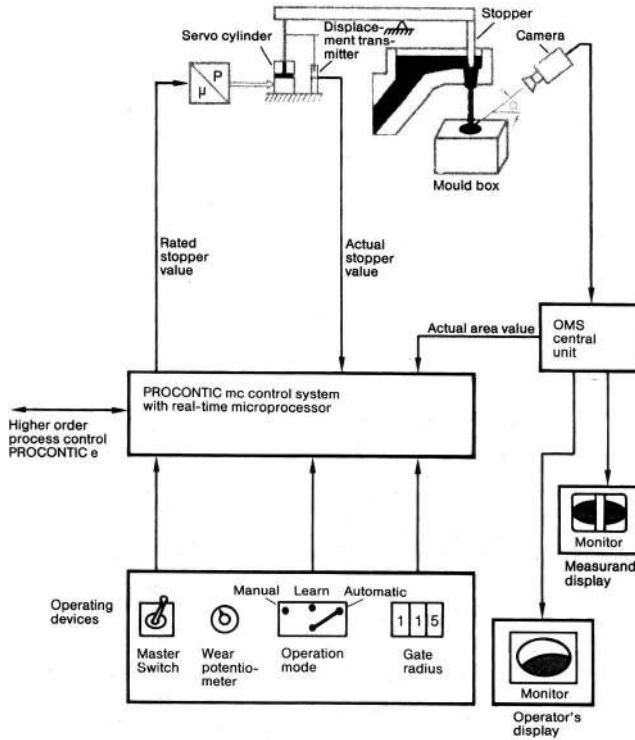
Figure 8: Schematic diagram of casting level control system Optipour
