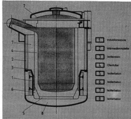
Figure 12: Crucible-type storage furnace with short coil
