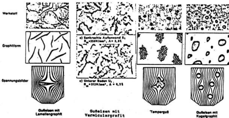
Figure 1: Structure, graphite form and tension patterns of various cast iron materials
