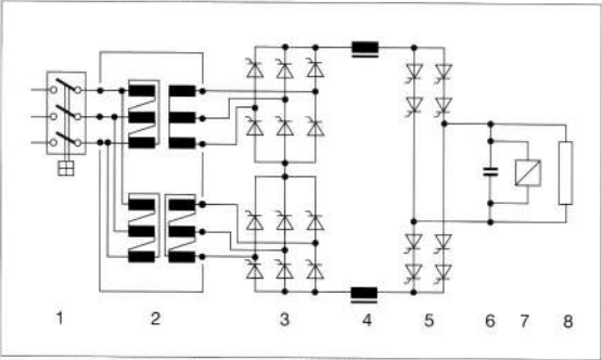
Figure 2: Block diagram of a thyristor converter (12-pulse)
