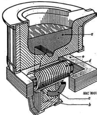
Figure 3-44 Schematic section of an induction furnace with vertically arranged channel
