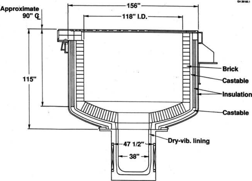
Fig. 1: Coreless inductor furnace
