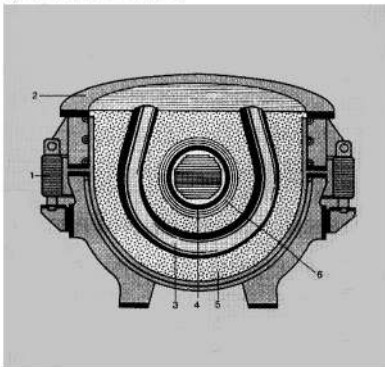
Fig. 2: Elementary diagram of channel-type inductors
