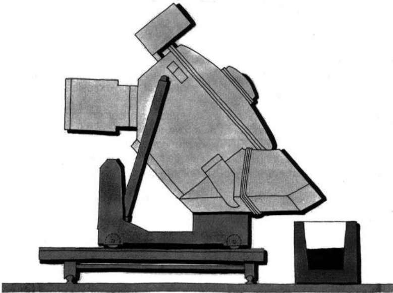
Fig. 2: Tilting of the PRESSPOUR ® -furnace for total emptying
