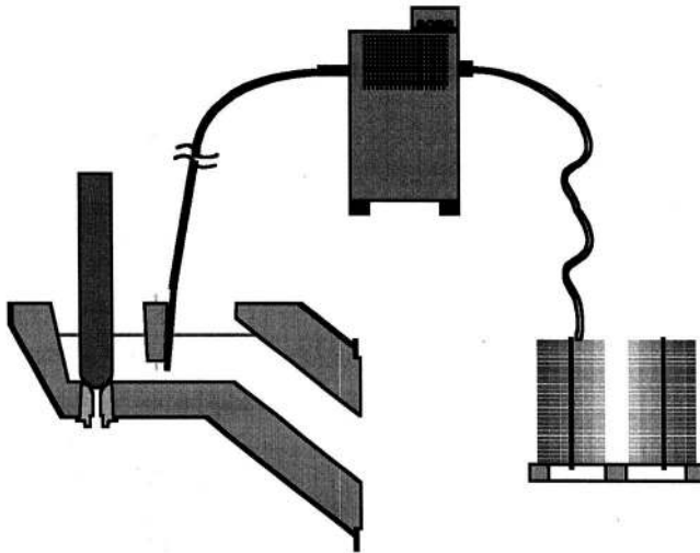
Fig. 9: Wire inoculation in the pouring spout
