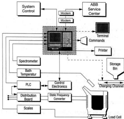
Fig. 6: Tele-Service
