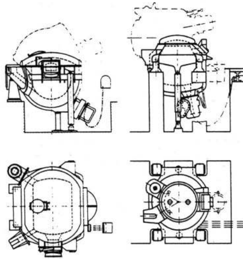
Figure 2: Design of vat-shaped (IRV) and crucible-shaped (IRT) channel-type furnaces
