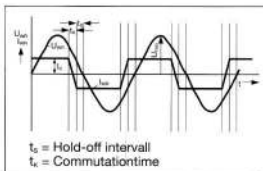
Figure 5: Time characteristic of the converter voltage U_m and the converter current I_m
