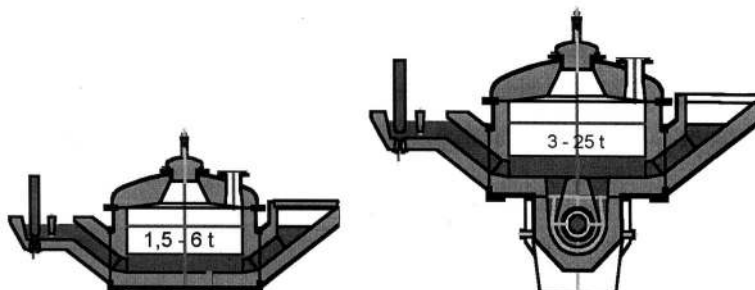
Fig. 4: The unheated Pouromat® System and the heated Presspour® System
