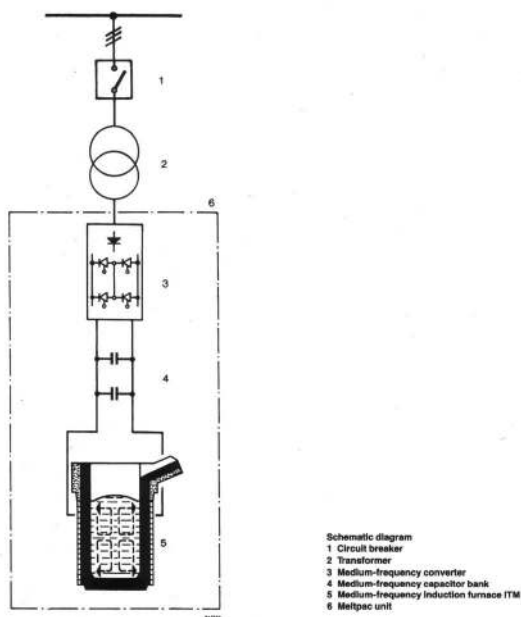
Fig. 1: Schematic set-up of an MF melting system (ABB Design)
