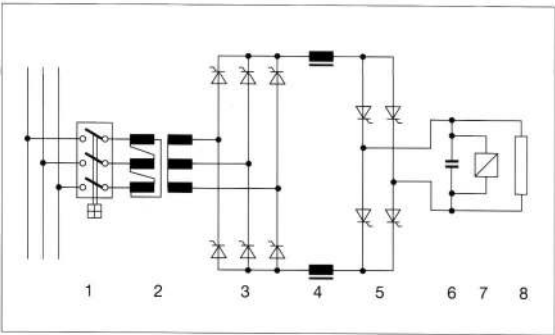
Figure 1: Block diagram of a thyristor (6-pulse)
