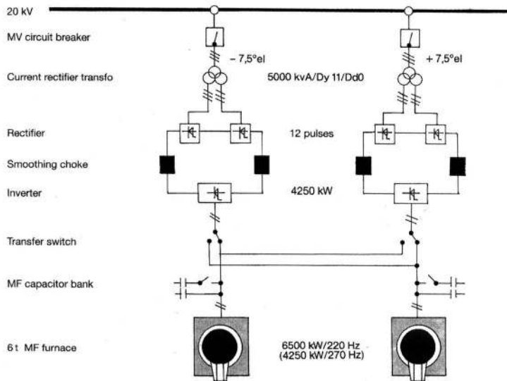
Fig. 11: MF power supply system 6,5/4,25 MW for 2 MF furnaces of 6 t each
