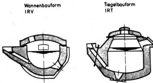
Figure 3: Cross-section through the vessel of a tub-shaped (left) and crucible-shaped channel-type furnace tub shape (IRV) - crucible shape (IRT)
