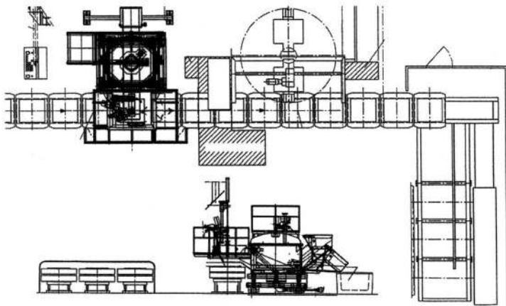
Fig. 1: POUROMAT configuration of the casting line
