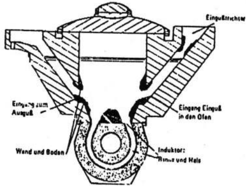
Figure 1: Slag deposit areas in a pressure casting furnace for Mg-treated spheroidal graphite cast iron
