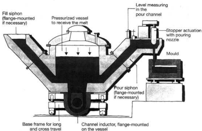
Fig. 1: Pressurized ABB pouring furnace PRESSPOUR®
