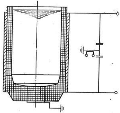
Figure 113. Crucible monitoring by means of bottom electrodes and soft central earthing of the coil [99].
