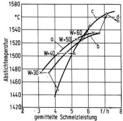
Figure 34. Iron temperature in relation to wind volume and added oil, coke percentage = 10% a without oil, b 50-60 l oil / h, c 90 l oil / h, d 120 l oil / h
