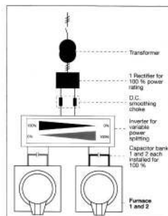
Figure 6: TWIN POWER circuit
