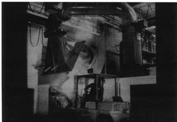
Figure 5: Magnesium treatment during tapping from the 40 t crucible-type furnace
