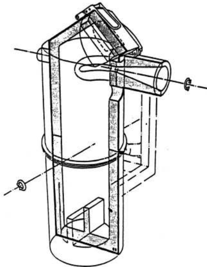
Figure 2: Converter for production of spheroidal graphite cast iron
