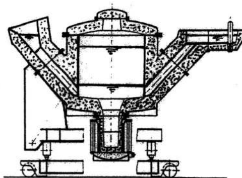
PRESSPOUR® casting furnace with flanged crucible inductor, usable capacity 5 t, converter performance for crucible inductor 350 kW at 260 Hz.
