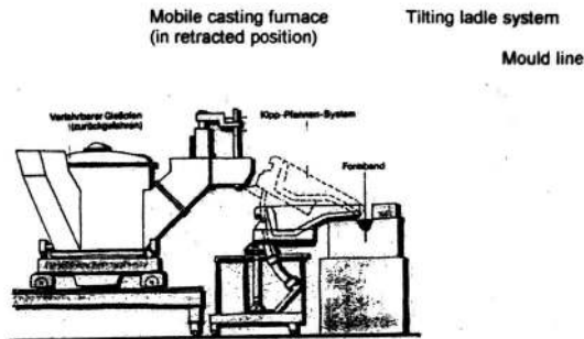
Figure 16: Tilting ladle system with the PRESSPOUR® casting furnace
