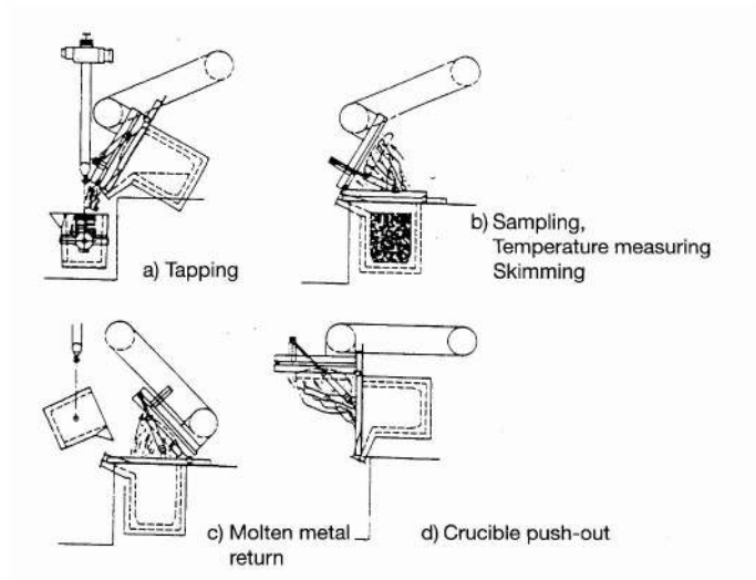
Fig. 2 a): Function of flue gas exhaust hood for various operating conditions
