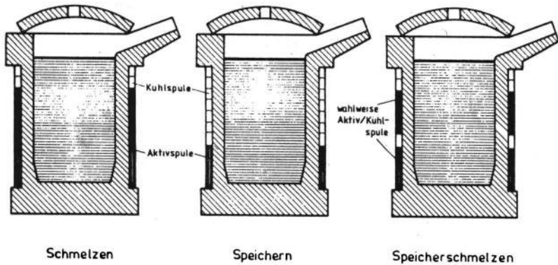
Figure 8: Schematic diagrams of crucible-type melting furnace (left) and crucible-type storage furnace with single coil (centre) and with reversible coil (right)
