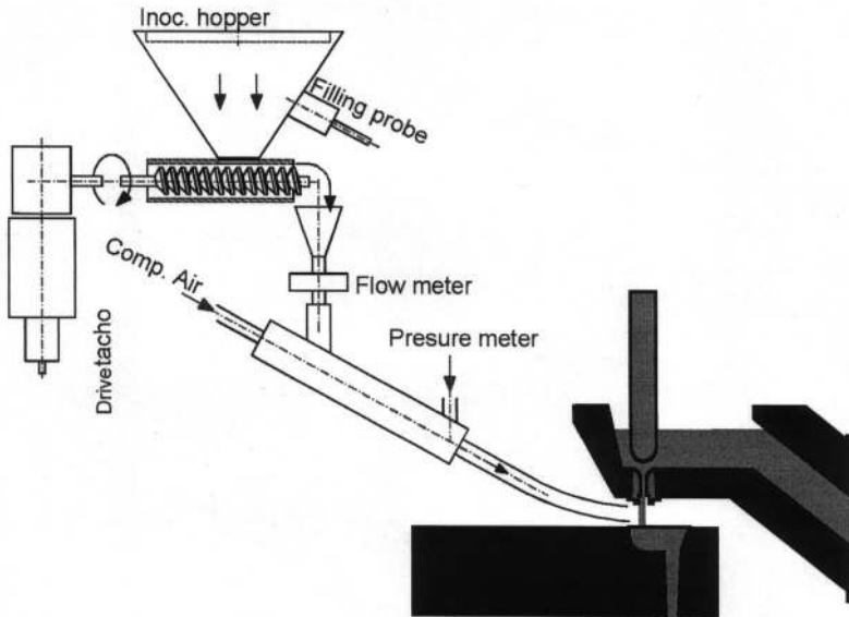
Fig. 8: Diagram of pouring stream inoculation with the necessary monitoring system.
