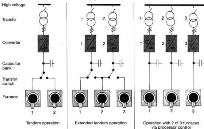
Fig. 10: Schematics of melting systems and associated power supply
