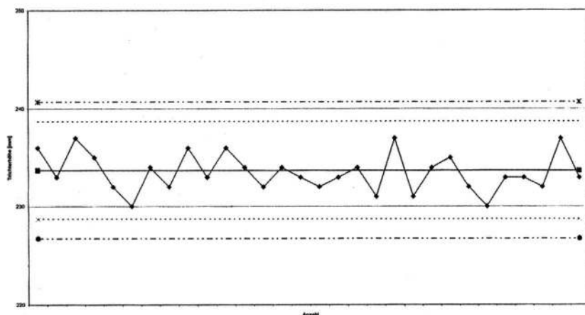
Fig. 7: Measured spoon cup heights of 30 pouring sequences (B)
