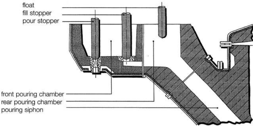
Fig. 10: Isopour® process
