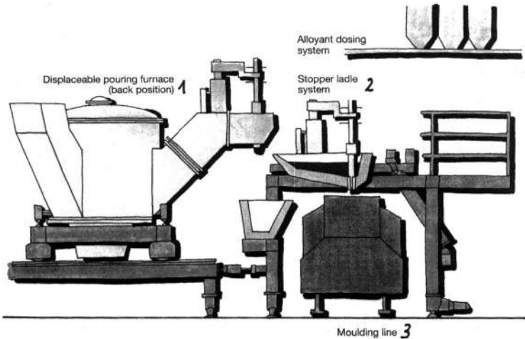
Fig. 15: Stopper ladle pouring system with pouring furnace and ladles arranged on a car 1 Pouring furnace in retracted position 2 Stopper ladle system 3 Moulding chain
