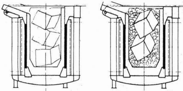
Figure 16: Charging of medium-frequency melting furnaces in charging/melting mode with large sized and bulky charge material
