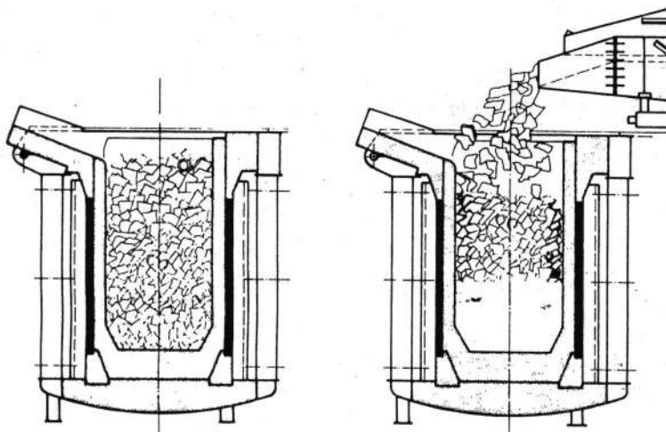
Figure 15: Charging of medium-frequency melting furnaces in charging/melting mode with normal sized and small charge material
