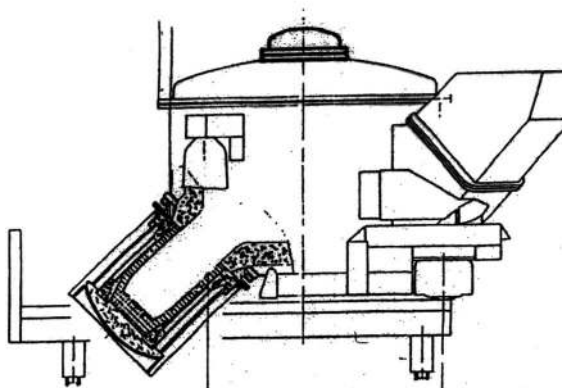
PRESSPOUR® casting furnace with crucible inductor flanged at 45°.
