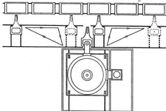
Figure 2: Pouring ladle carousel with 8 tonne casting furnace for automatic casting of continuously moving moulds
